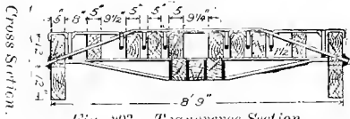
Fig. 293. Transverse Section.
